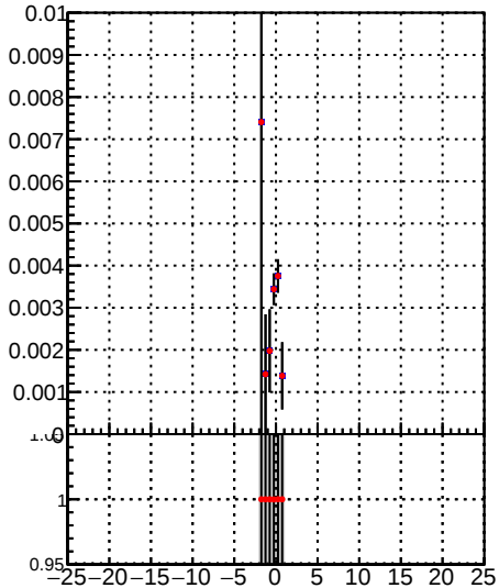
Pileup rate vs \Delta y
