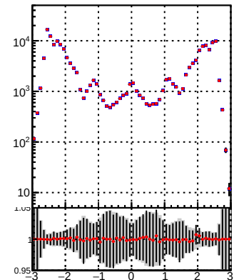
—•— DQM_TT_mkFit-DQM_init_orig —•— DQM_TT_mkFit-DQM_init_modi3
