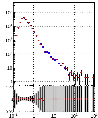
—•— DQM_TT_mkFit-DQM_init_orig —•— DQM_TT_mkFit-DQM_init_modi3
