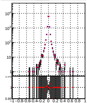
DQM_TT_mkFit-DQM_init_orig DQM_TT_mkFit-DQM_init_modi3
