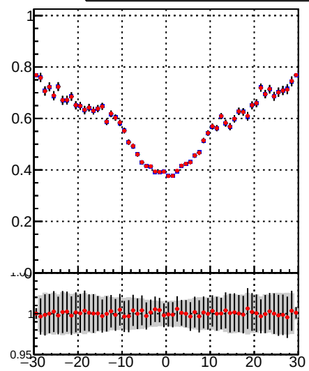
—•— DQM_TT_mkFit-DQM_init_orig —•— DQM_TT_mkFit-DQM_init_modi3
