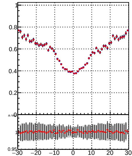
—•— DQM_TT_mkFit-DQM_init_orig —•— DQM_TT_mkFit-DQM_init_modi3
