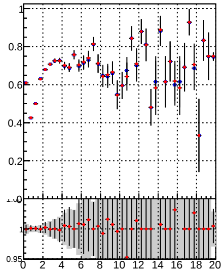
Fake rate vs. —•— DQM_TT_mkFit-DQM_init_orig —•— DQM_TT_mkFit-DQM_init_modi3
