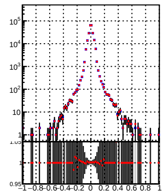
Legend: \blacksquare DQM_TT_mkFit-DQM_init_orig \bullet DQM_TT_mkFit-DQM_init_modi3
