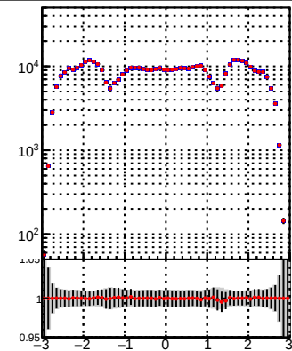
—●— DQM_TT_mkFit-DQM_init_orig —●— DQM_TT_mkFit-DQM_init_modi3
