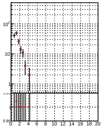
N of reco track vs. \chi^2 for DQM TT mkFit-DQM_init_orig and DQM TT mkFit-DQM_init_modi3
