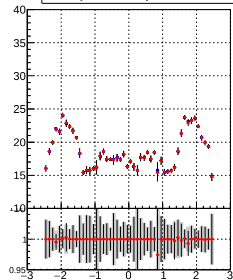
— DQM_TT_mkFit-DQM_init_orig — DQM_TT_mkFit-DQM_init_mod3
