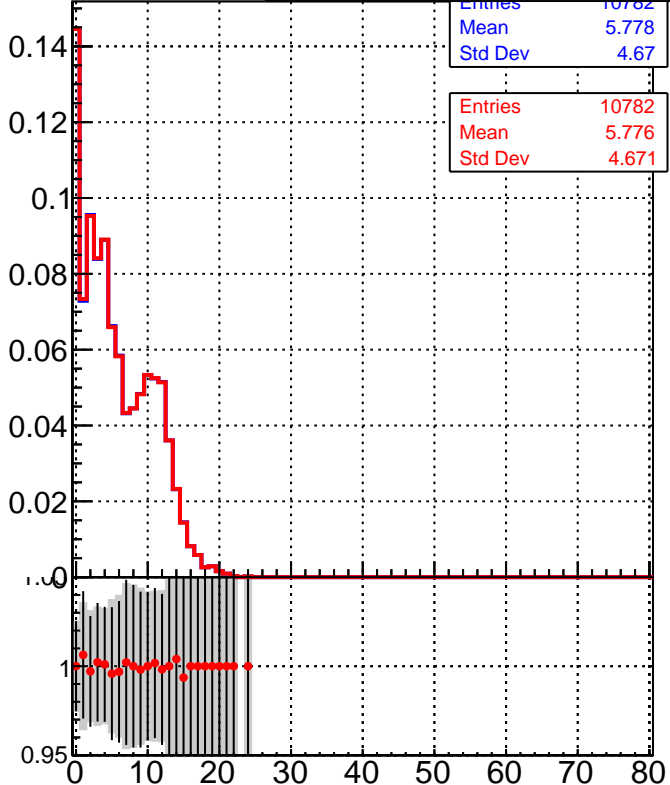
■ DQM_TT_mkFit-DQM_init_orig ● DQM_TT_mkFit-DQM_init_modi3
