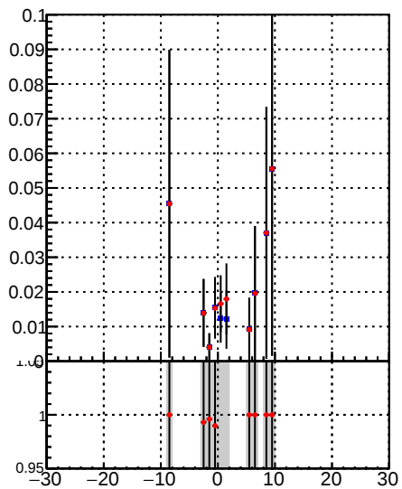
—●— DQM_TT_mkFit-DQM_init_orig —●— DQM_TT_mkFit-DQM_init_modi3
