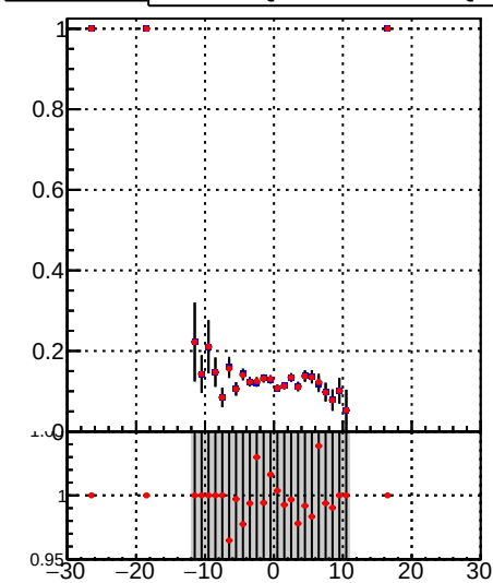
—•— DQM_TT_mkFit-DQM_init_orig —•— DQM_TT_mkFit-DQM_init_modi3
