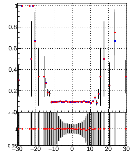
—•— DQM_TT_mkFit-DQM_init_orig —•— DQM_TT_mkFit-DQM_init_modi3
