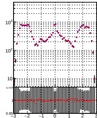
—•— DQM_TT_mkFit-DQM_init_orig —•— DQM_TT_mkFit-DQM_init_modi3
