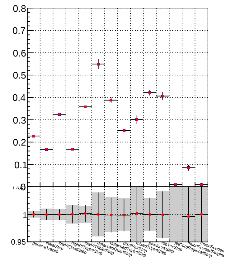
Duplicates rate vs collection Legend: DQM_TT_mkFit-DQM_init_orig (Blue square) DQM_TT_mkFit-DQM_init_modi3 (Red circle)
