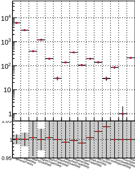
Number —●— DQM_TT_mkFit-DQM_init_modi3
