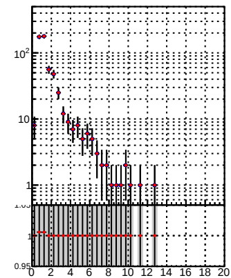
N of reco track vs. \chi^2 — mkFit-DQM_init_orig — mkFit-DQM_init_modi3
