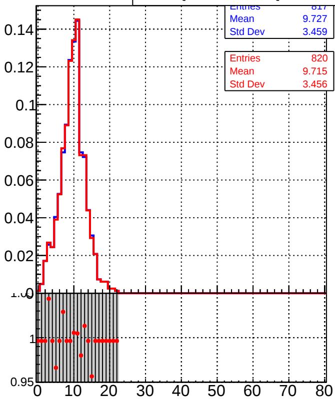
Legend: DQM_TT_mkFit-DQM_init_orig (Blue line with squares) DQM_TT_mkFit-DQM_init_modi3 (Red line with circles)
