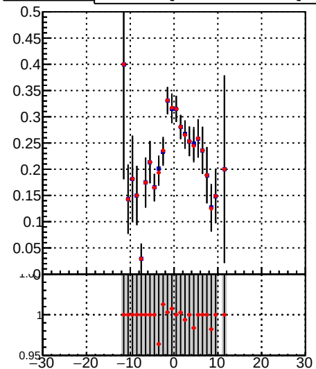
Fake rate vs v Legend: DQM_TT_mkFit-DQM_init_orig (grey line with blue dots) DQM_TT_mkFit-DQM_init_modi3 (red line with red dots)
