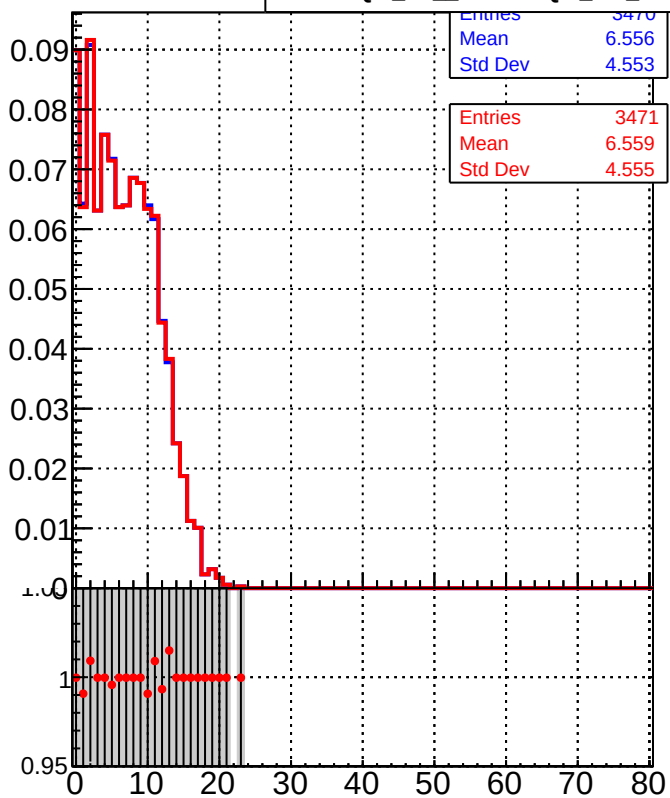
Legend for bottom row: ■ DQM_TT_mkFit-DQM_init_orig ● DQM_TT_mkFit-DQM_init_modi3
