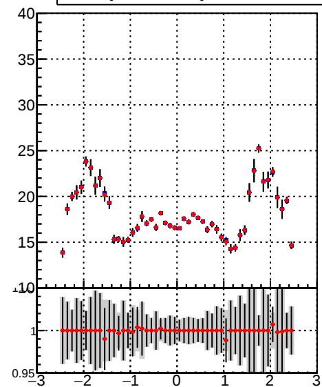
mean hit DQM_TT_mkFit-DQM_init_orig DQM_TT_mkFit-DQM_init_mod3
