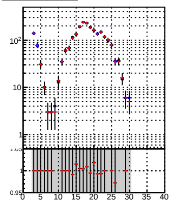
—•— DQM_TT_mkFit-DQM_init_orig —•— DQM_TT_mkFit-DQM_init_modi3
