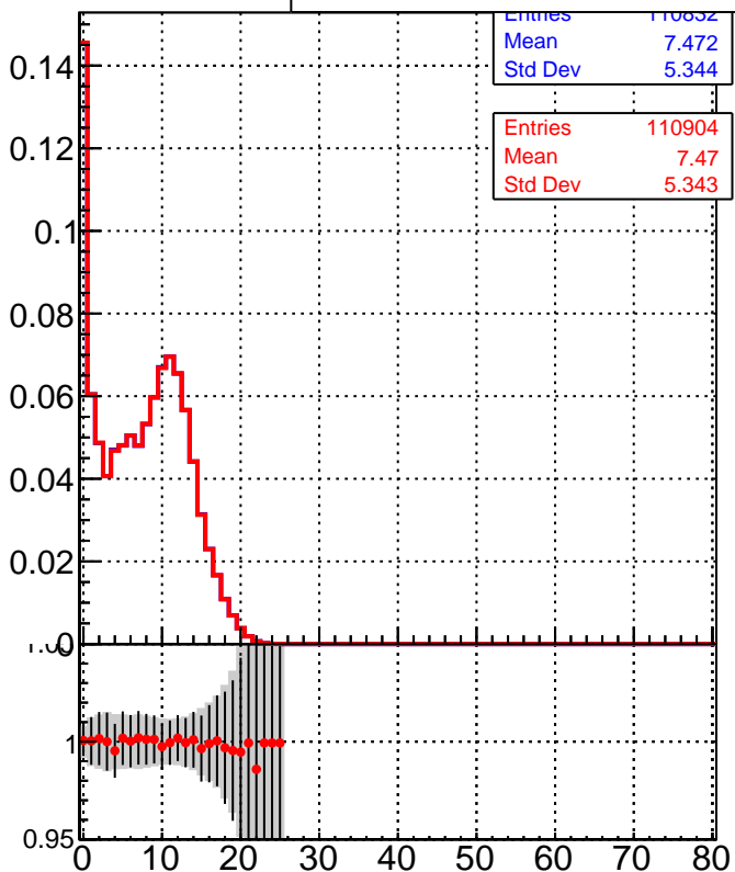
— DQM_TT_mkFit-DQM_init_orig —• DQM_TT_mkFit-DQM_init_modi3
