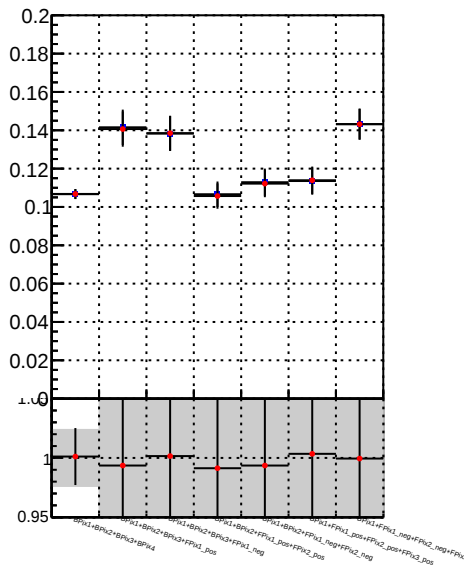
Fake rate vs. \text{DQM\_TT\_mkFit-DQM\_init\_orig} \text{DQM\_TT\_mkFit-DQM\_init\_modi3}
