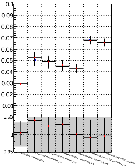
Fake rate vs. —•— DQM TT mkFit-DQM_init_orig —•— DQM TT mkFit-DQM_init_modi3
