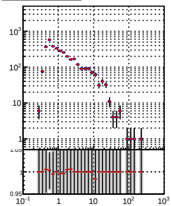
—●— DQM_TT_mkFit-DQM_init_orig —●— DQM_TT_mkFit-DQM_init_modi3
