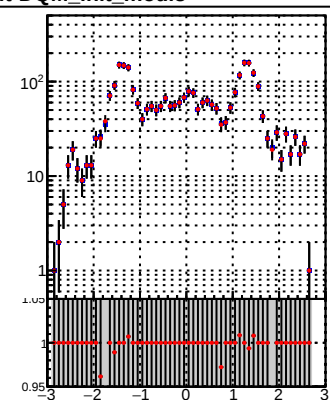
—●— DQM_TT_mkFit-DQM_init_orig —●— DQM_TT_mkFit-DQM_init_modi3
