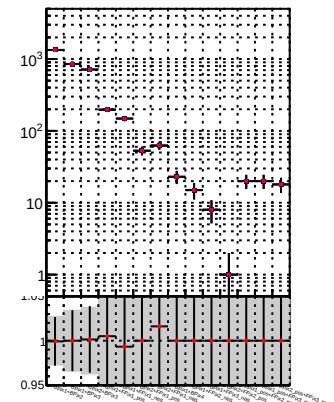
N of reco track vs. \chi^2 vs. \chi^2 vs. \chi^2
