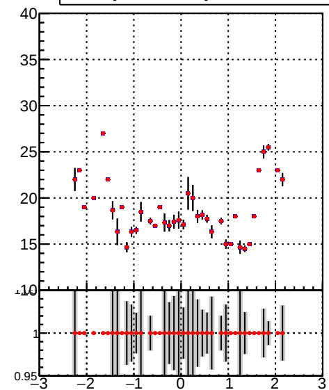
mean hit Legend: DQM_TT_mkFit-DQM_init_orig DQM_TT_mkFit-DQM_init_modi3
