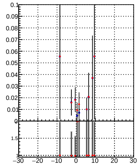
—●— DQM_TT_mkFit-DQM_init_orig —●— DQM_TT_mkFit-DQM_init_modi3
