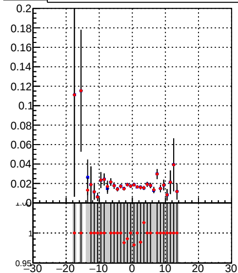
Efficiency vs. sim PV z — DQM_TT_mkFit-DQM_init_orig — DQM_TT_mkFit-DQM_init_modi3
