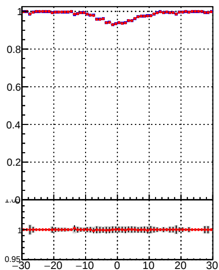
—●— DQM_TT_mkFit-DQM_init_orig —●— DQM_TT_mkFit-DQM_init_modi3
