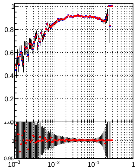
—•— DQM_TT_mkFit-DQM_init_orig —•— DQM_TT_mkFit-DQM_init_modi3
