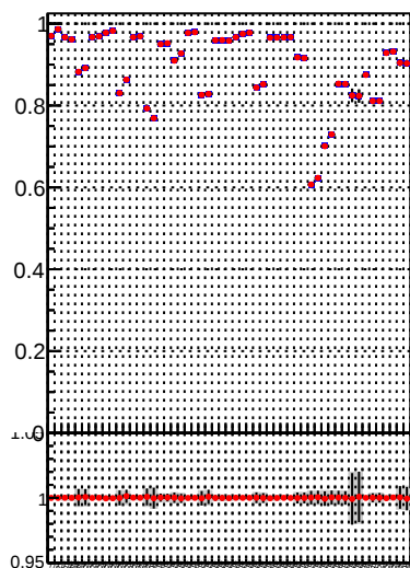
Fake rate vs. DQM_TT_mkFit-DQM_init_orig DQM_TT_mkFit-DQM_init_mod3
