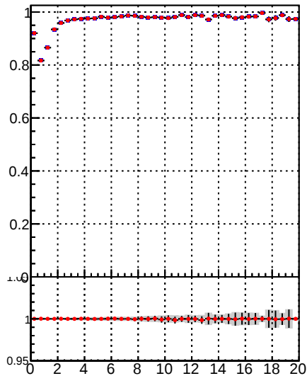
Fake rate vs. DQM_TT_mkFit-DQM_init_orig DQM_TT_mkFit-DQM_init_mod3
