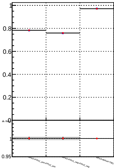
Fake rate vs. DQM_TT_mkFit-DQM_init_orig DQM_TT_mkFit-DQM_init_modi3
