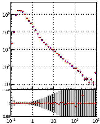
—●— DQM_TT_mkFit-DQM_init_orig —●— DQM_TT_mkFit-DQM_init_modi3
