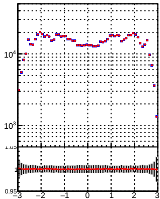
—●— DQM_TT_mkFit-DQM_init_orig —●— DQM_TT_mkFit-DQM_init_modi3
