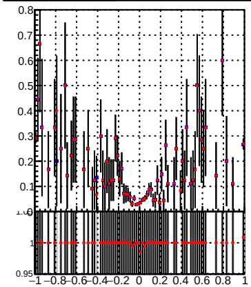
Efficiency vs Dxy(PV) Legend: DQM_TT_mkFit-DQM_init_orig DQM_TT_mkFit-DQM_init_mod3
