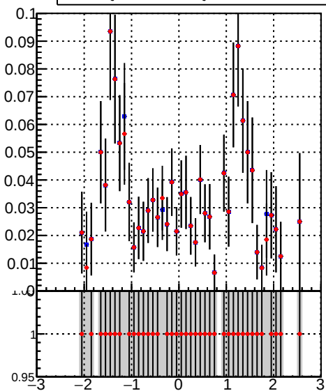
DQM_TT_mkFit-DQM_init_orig DQM_TT_mkFit-DQM_init_modi3
