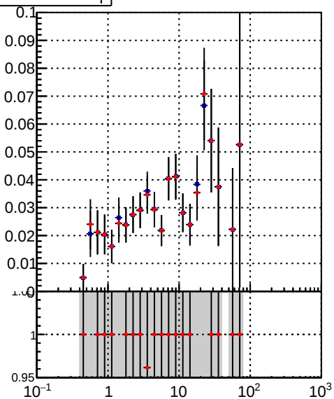
DQM_TT_mkFit-DQM_init_orig DQM_TT_mkFit-DQM_init_modi3
