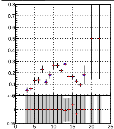
Efficiency vs hit Legend: DQM_TT_mkFit-DQM_init_orig DQM_TT_mkFit-DQM_init_modi3
