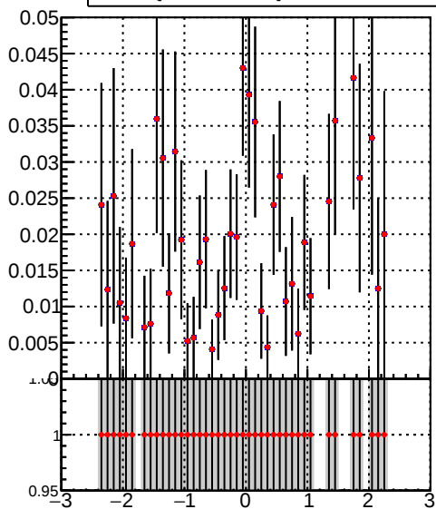
DQM_TT_mkFit-DQM_init_orig DQM_TT_mkFit-DQM_init_modi3
