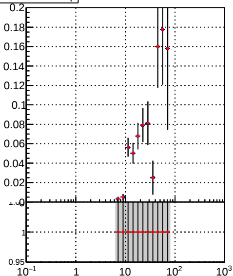
DQM_TT_mkFit-DQM_init_orig DQM_TT_mkFit-DQM_init_modi3
