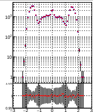
N of reco track vs \eta DQM_TT mkFit-DQM_init_orig DQM_TT mkFit-DQM_init_modi3
