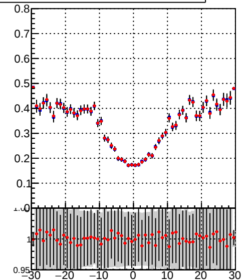
fake+duplicates vs vert r
