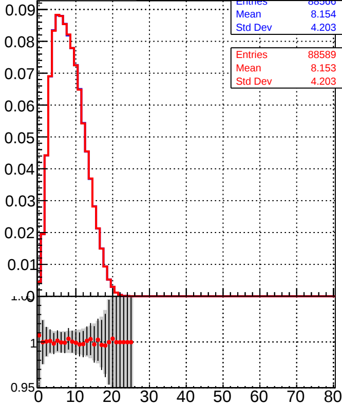
Legend: DQM_TT_mkFit-DQM_init_orig (grey histogram) DQM_TT_mkFit-DQM_init_modi3 (red line with markers)
