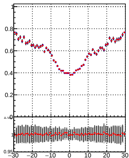
Fake rate vs d —■— DQM_TT_mkFit-DQM_init_orig —●— DQM_TT_mkFit-DQM_init_modi3
