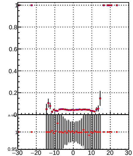
—●— DQM_TT_mkFit-DQM_init_orig —●— DQM_TT_mkFit-DQM_init_modi3
