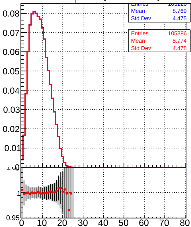
— DQM_TT_mkFit-DQM_init_orig — DQM_TT_mkFit-DQM_init_modi3
