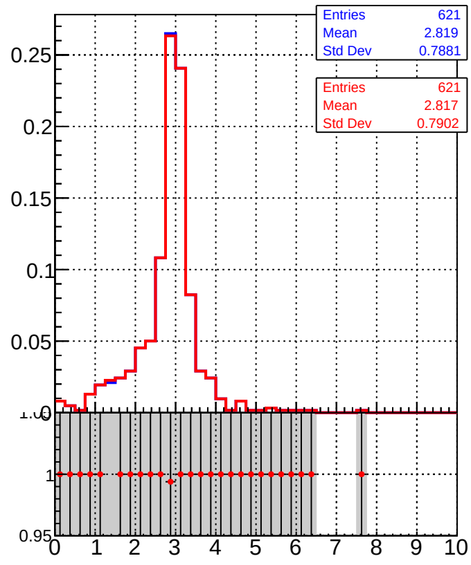
Legend: DQM_TT_mkFit-DQM_init_orig (grey histogram, blue line with points) DQM_TT_mkFit-DQM_init_modi3 (red line with points)
