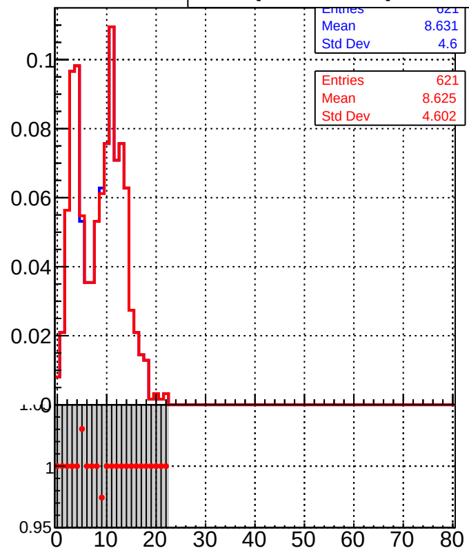
Legend: DQM_TT_mkFit-DQM_init_orig (grey histogram, blue line with points) DQM_TT_mkFit-DQM_init_modi3 (red line with points)
