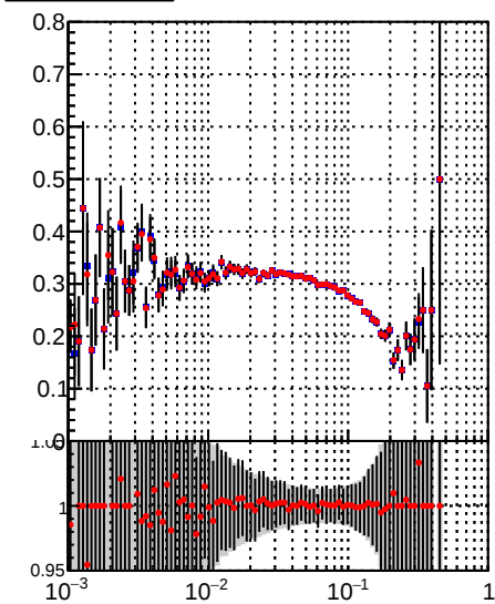
—•— DQM_TT_mkFit-DQM_init_orig —•— DQM_TT_mkFit-DQM_init_modi3
