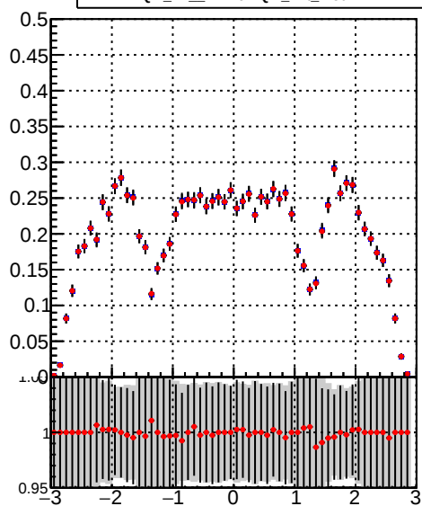
■ DQM_TT_mkFit-DQM_init_orig — DQM_TT_mkFit-DQM_init_modi2
