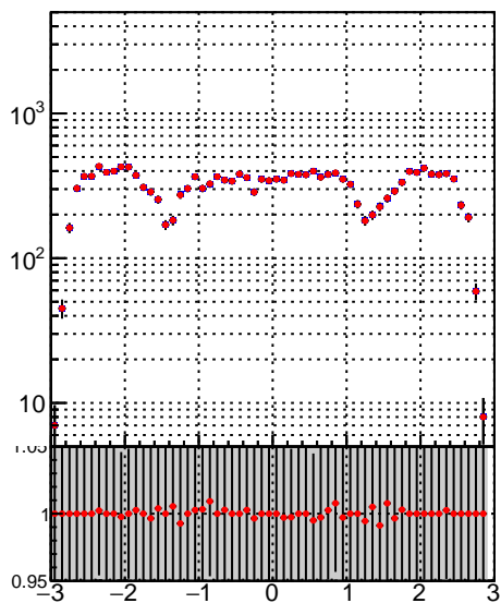
DQM_TT_mkFit-DQM_init_orig DQM_TT_mkFit-DQM_init_mod2
